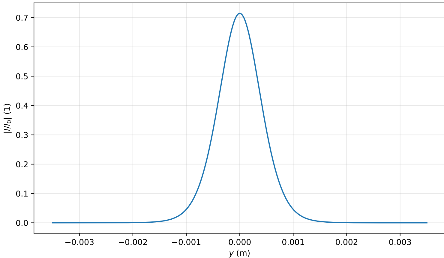
Intensity profile I(x=0, y, z=2.388)/I_0 , \text{Pin}=0.5\text{Pcr} , artificial time
